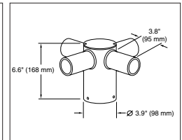
PT-4 (90) 90° Quad
