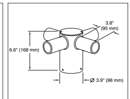
PT-4 (90) 90° Quad
