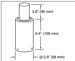
PT-1 Single
