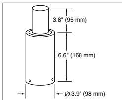
PT-1 Single
